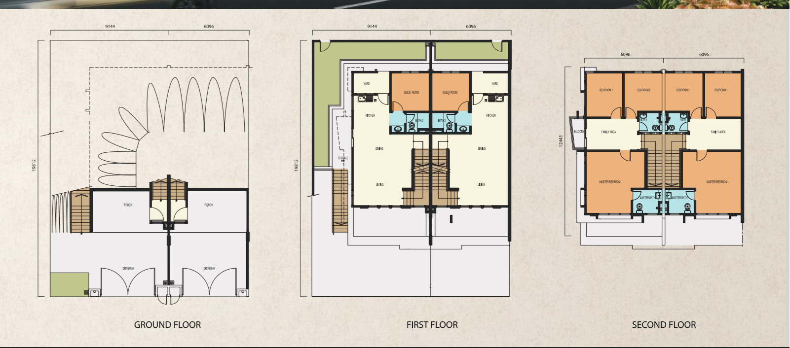
JADE 8 | 3-STOREY TERRACE HOUSE | 20' x 65' | 1,645 sq.ft. (Std Unit)
